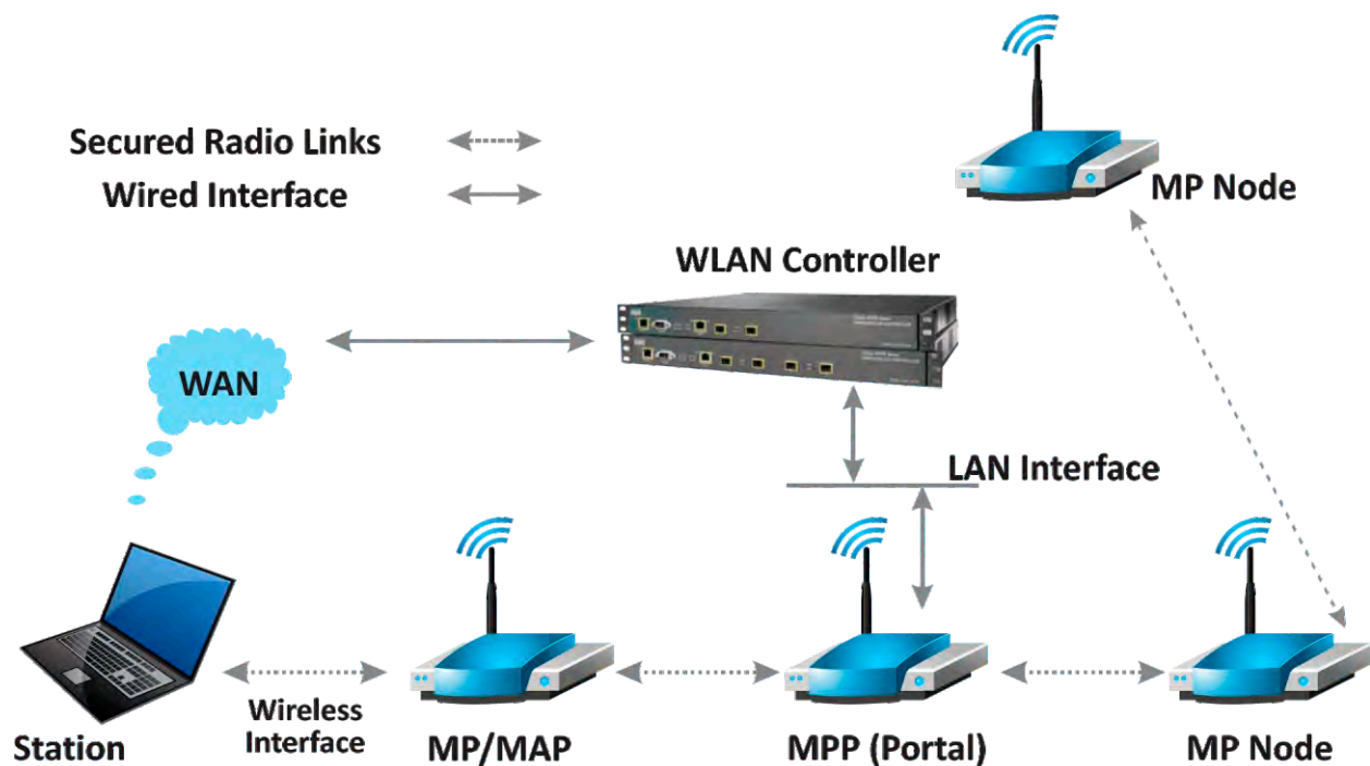
Configuring Mesh Node using WLAN Controller
